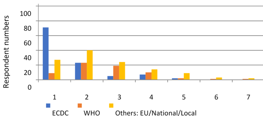
Figure 15: Categories of guidelines ranked 1-7 by respondents.
