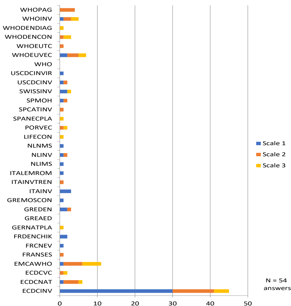
Figure 23: The best guidelines categories ranked from 1 to 3 by the respondent in terms of scale, in the respondent's local context.
