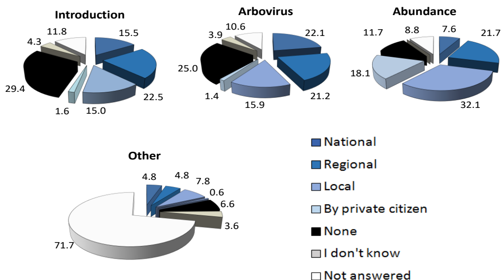
Figure 9: Control objectives at different geographic scales. Values are % respondents.
