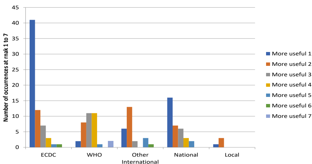
Figure 16: Guidelines categories ranked in terms of usefulness.
