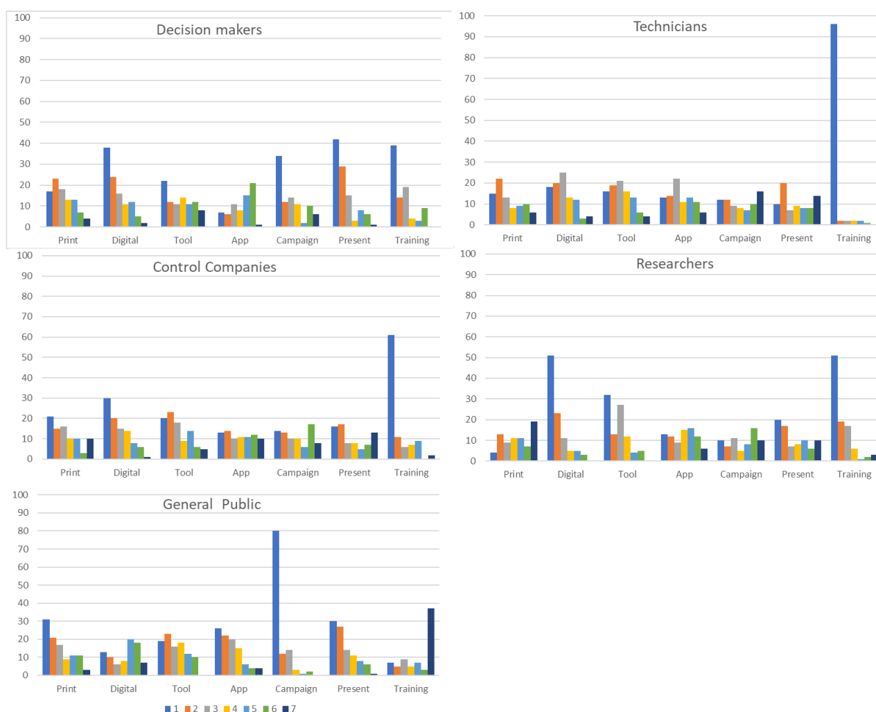
Figure 18: Most appropriate tools for dissemination of Guidelines to different user groups.
