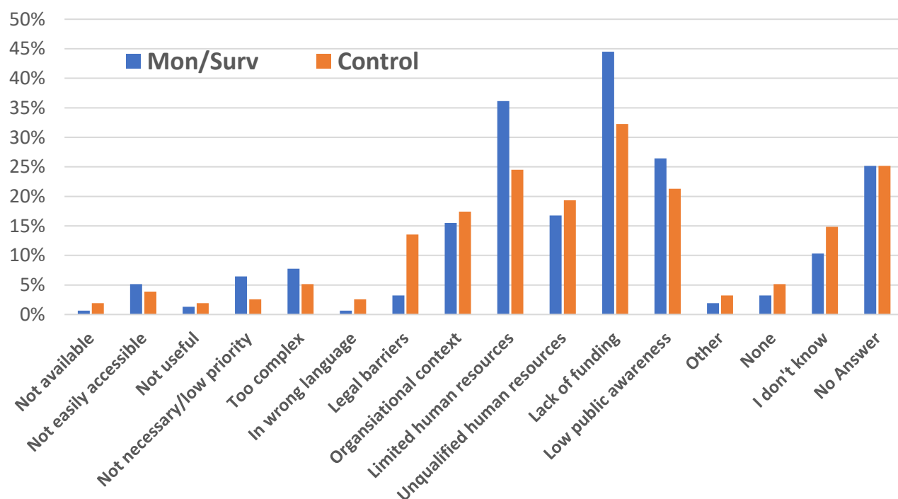
Figure 17: Constraints to use guidelines while implementing AIM surveillance and control.
