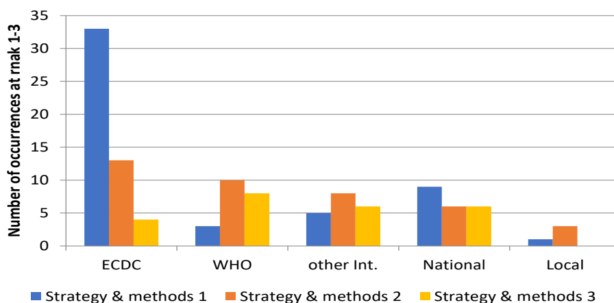
Figure 24: The best guidelines categories ranked from 1 to 3 by the respondent in terms of strategy and methods, in the respondent's local context.
