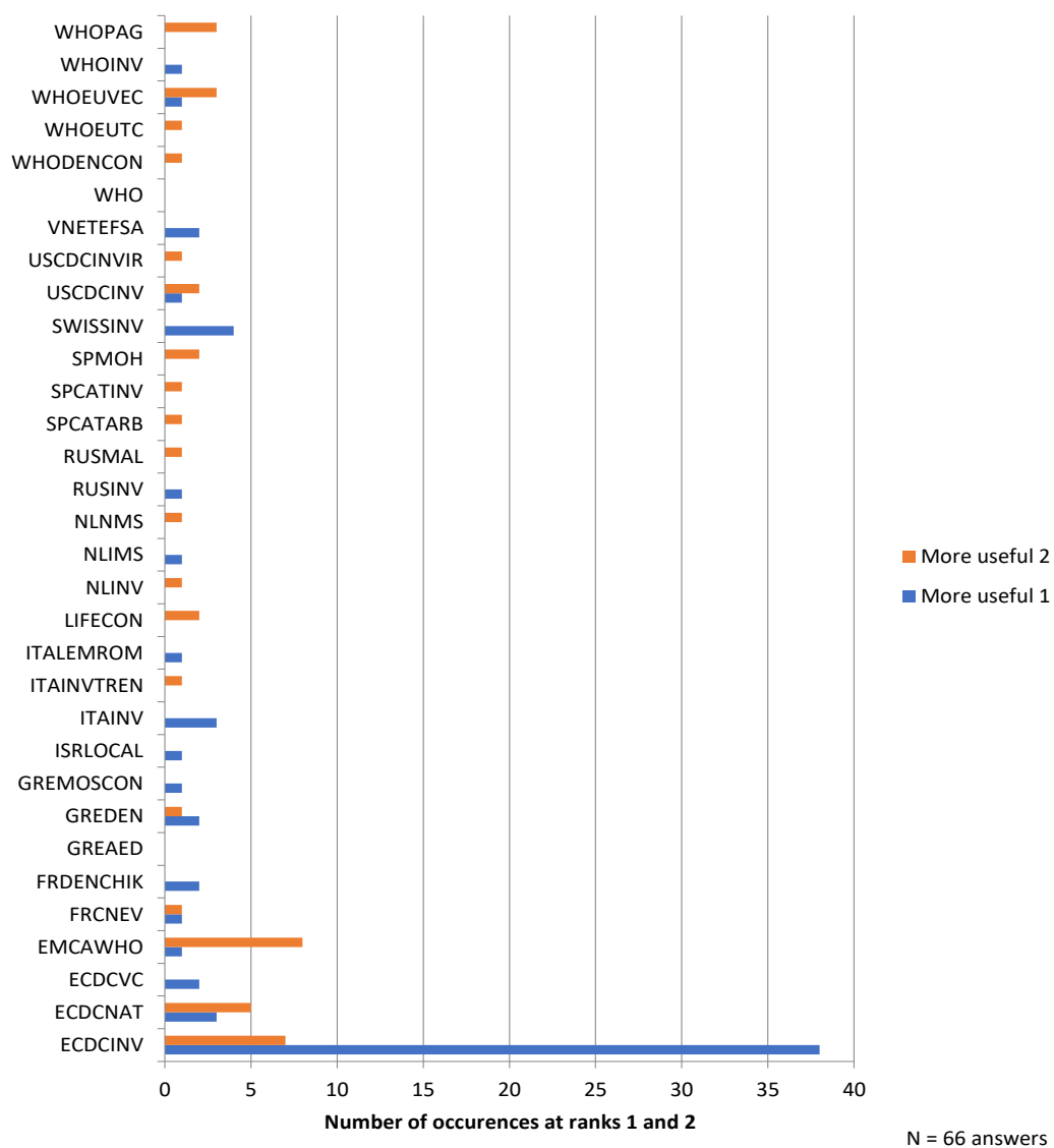
Figure 19: Guidelines ranked at 1 st and 2 nd place by the respondent in terms of usefulness, in the respondent's local context.
