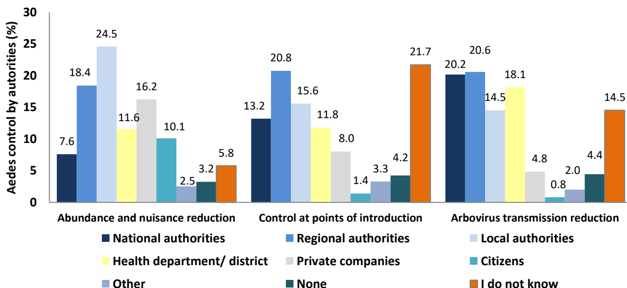
Figure 10: Implementing institutions for different control objectives. Values are % respondents.
