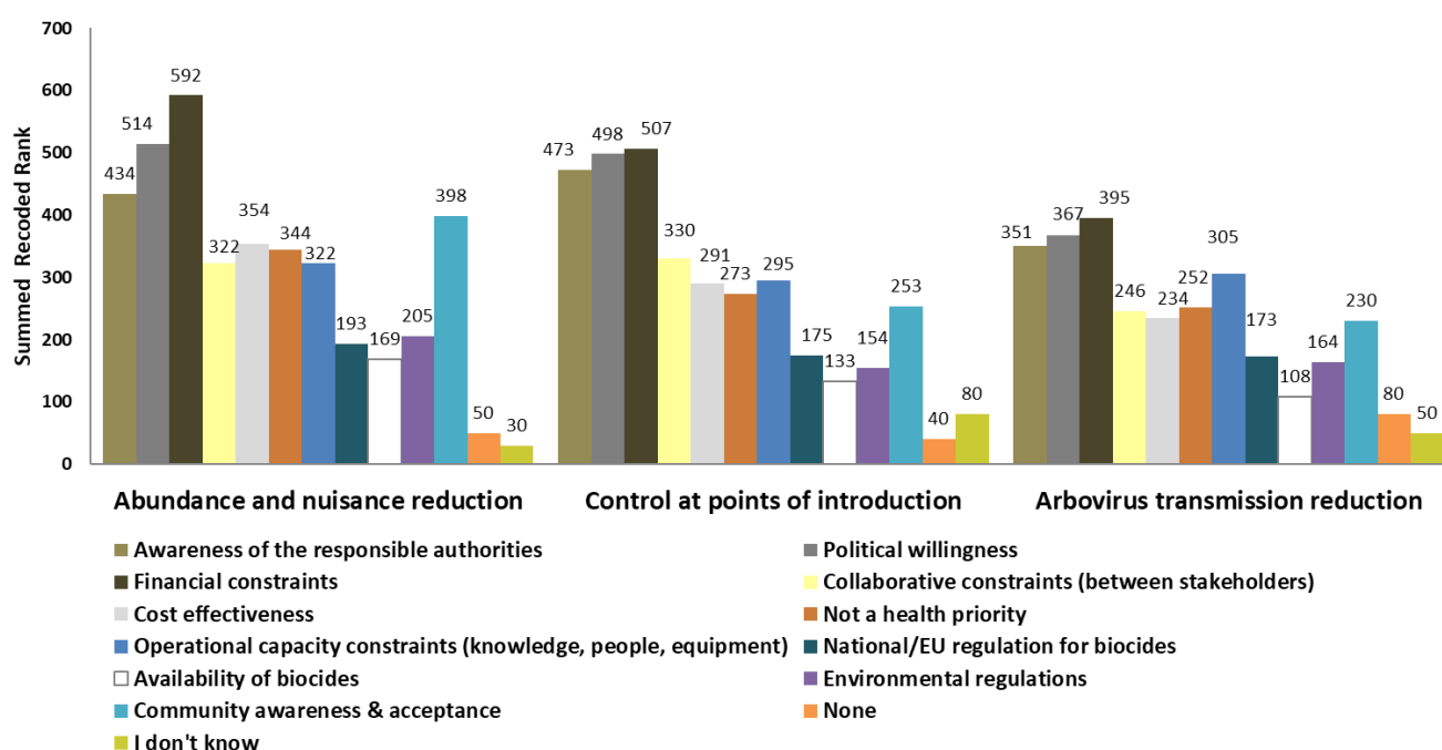
Figure 12: Reported constraints to control activities. Values are summed ranks, recoded as 1 st =10 points, 2 nd =5 points and 3 rd =1 point.
