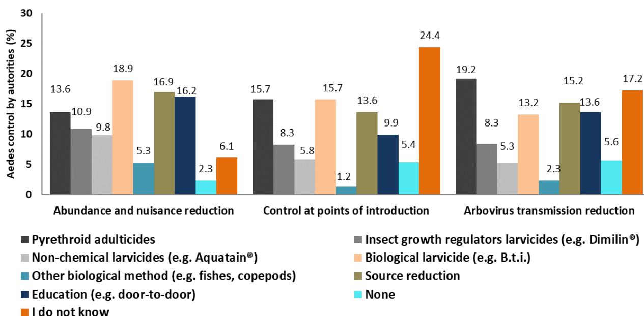
Figure 11: Methods used in control activities. Values are % respondents.
