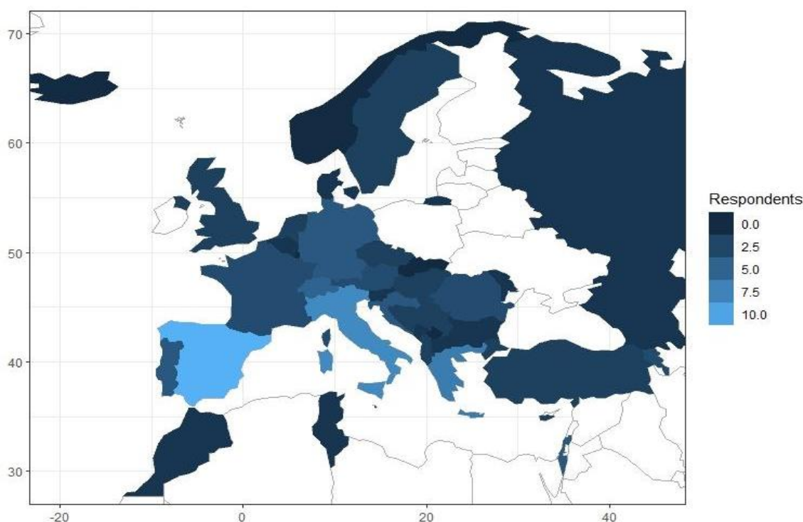
Figure 3: Number of respondents involved in surveillance per country. Countries in white not part of Action
